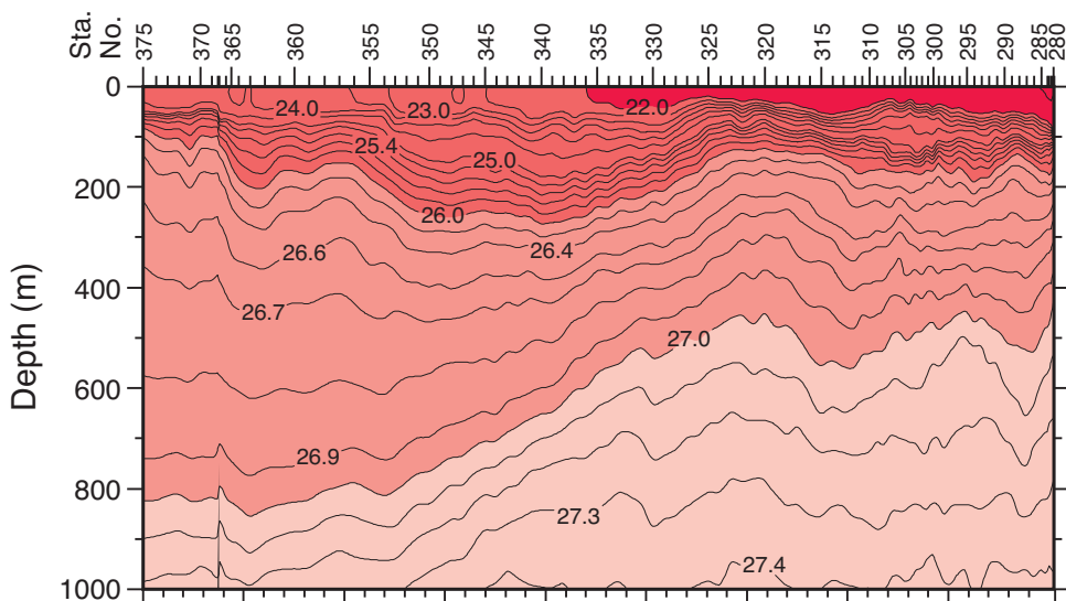
\sigma_0 (red), \sigma_2 (green), \sigma_4 (blue) ( \text{kg/m}^3 ) for I8N 80°E
