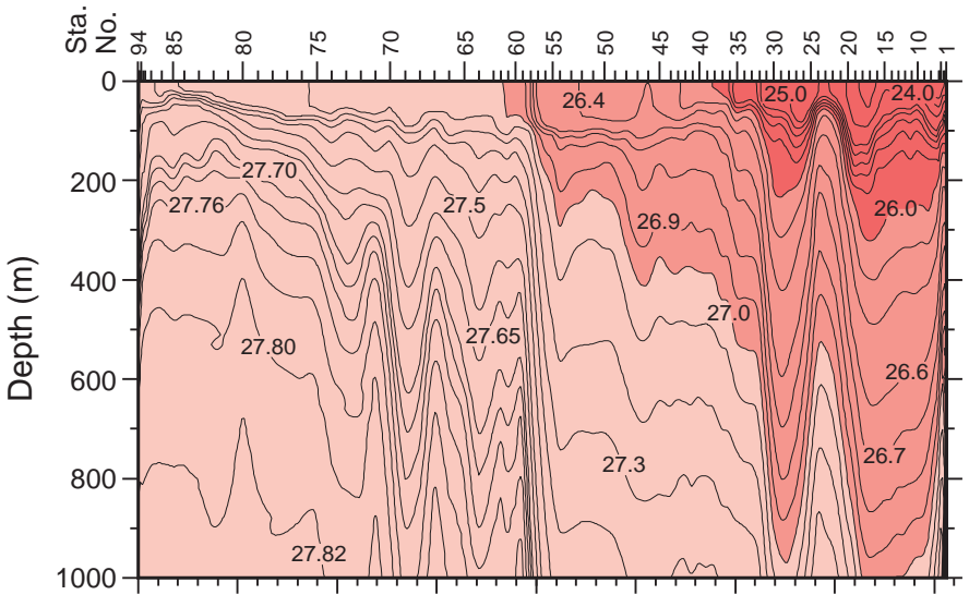
\sigma_0 (red), \sigma_2 (green), \sigma_4 (blue) ( \text{kg/m}^3 ) for I06 30°E
