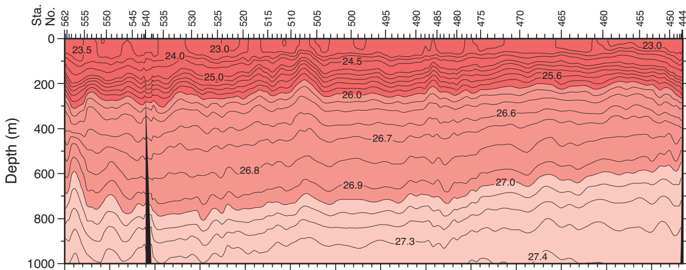
\sigma_0 (red), \sigma_2 (green), \sigma_4 (blue) kg/m 3 for I03 20°S
