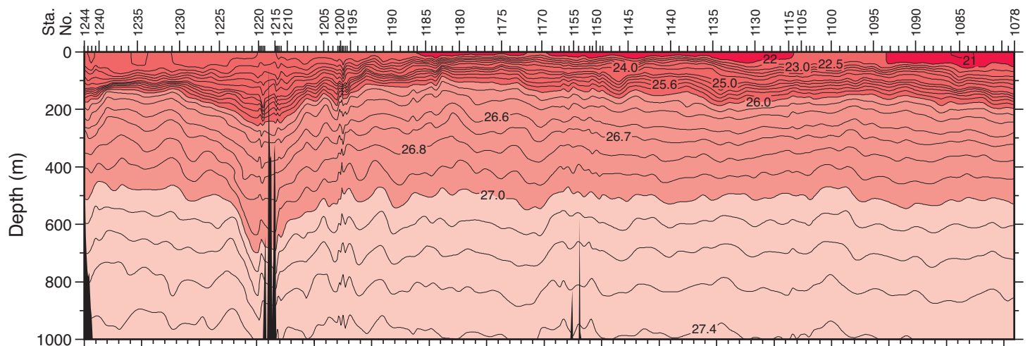
\sigma_0 (red), \sigma_2 (green), \sigma_4 (blue) (kg/m 3 ) for I02 8°S
