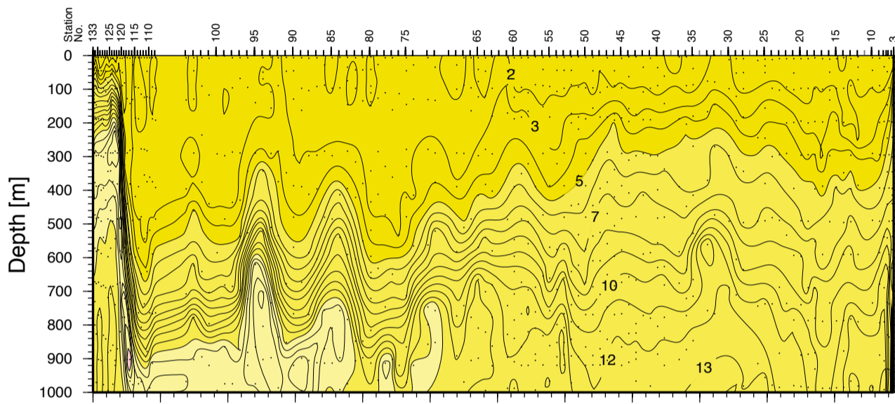
Silicate [ \mu\text{M}/\text{kg} ] for A03 36° N
