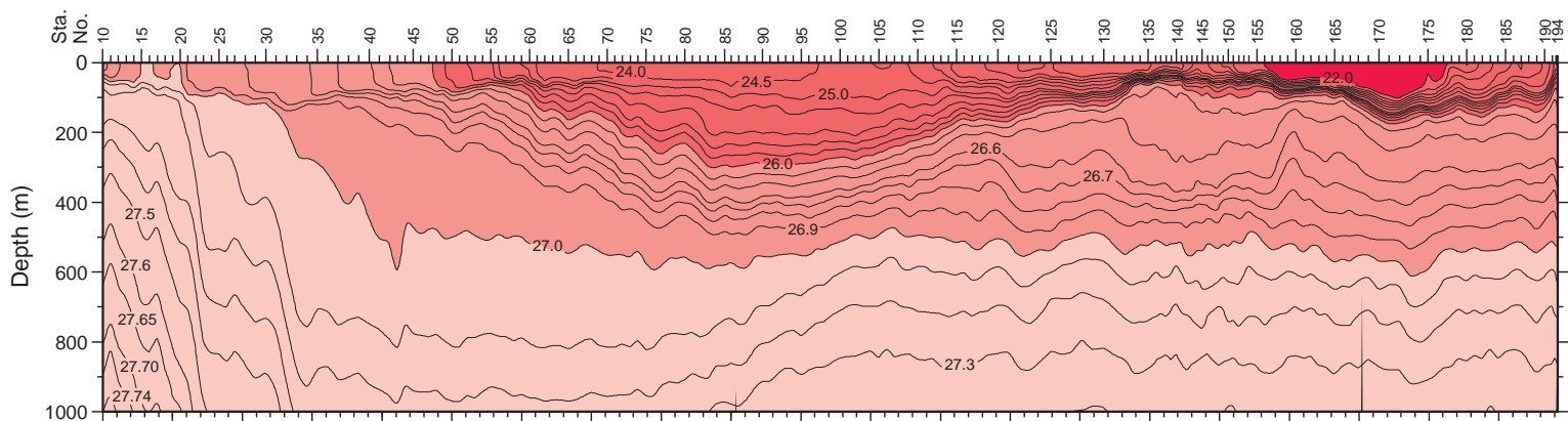
\sigma_0 (red), \sigma_2 (green), \sigma_4 (blue) for P18 105°W
