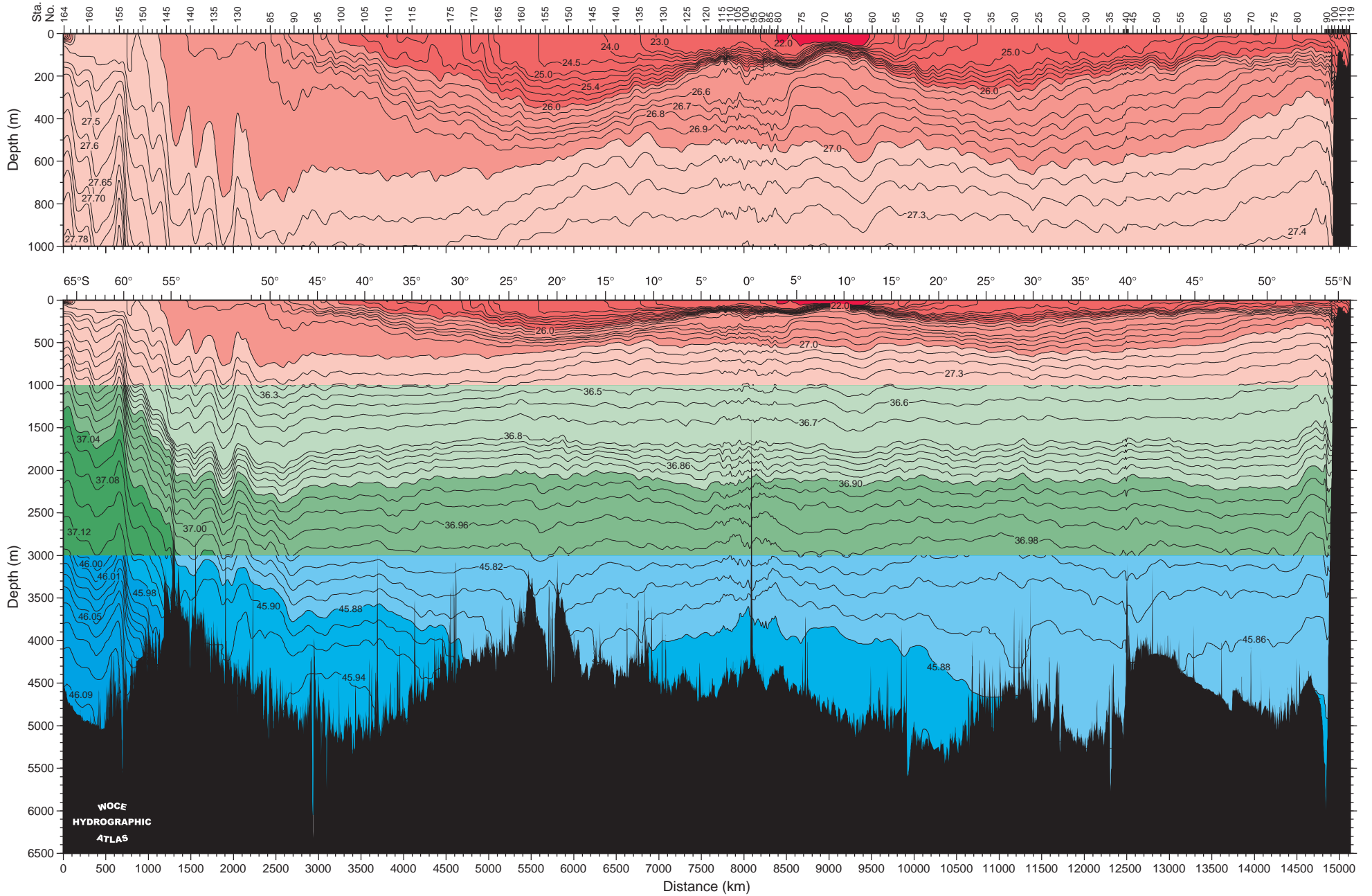
\sigma_0 (red), \sigma_2 (green), \sigma_4 (blue) for P17 135°W
