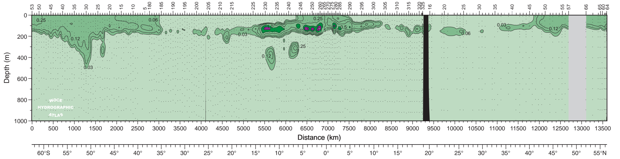
Nitrite ( \mu\text{mol/kg} ) for P16 150°W
