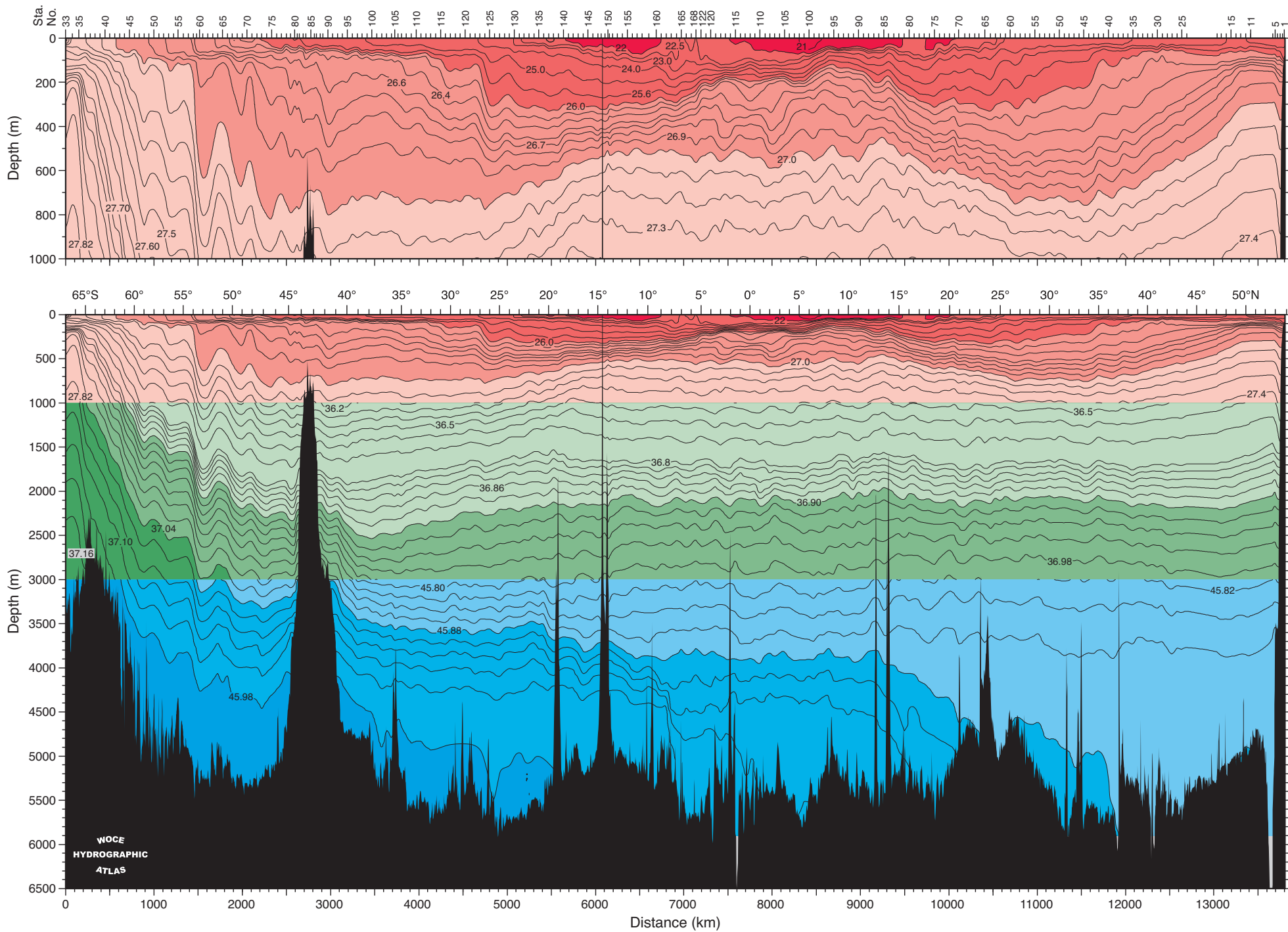
\sigma_0 (red), \sigma_2 (green), \sigma_4 (blue) for P15 165°W
