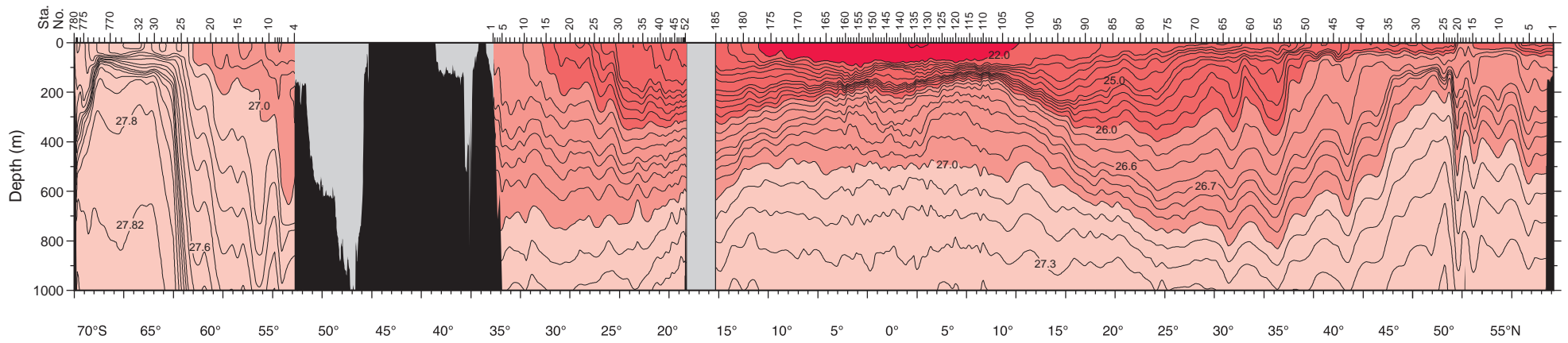
\sigma_0 (red), \sigma_2 (green), \sigma_4 (blue) for P14 179°E
