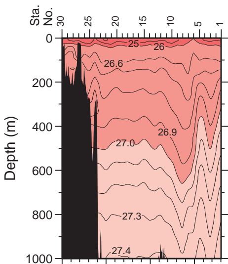
\sigma_0 (red), \sigma_2 (green), \sigma_4 (blue) for P01W Okhotsk Sea
